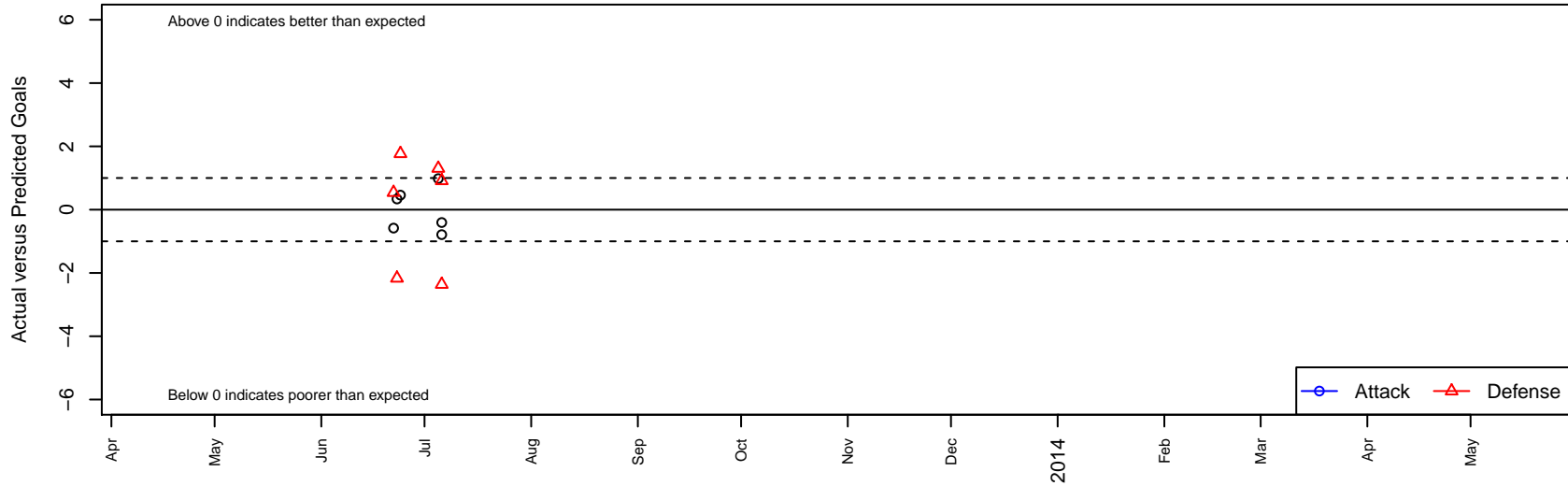
Bozeman Blitz B99 Dots are actual minus expected GF (blue circles) and GA (red triangles). Blue line is smoothed change in attack strength. Red is smoothed change in defense strength.
